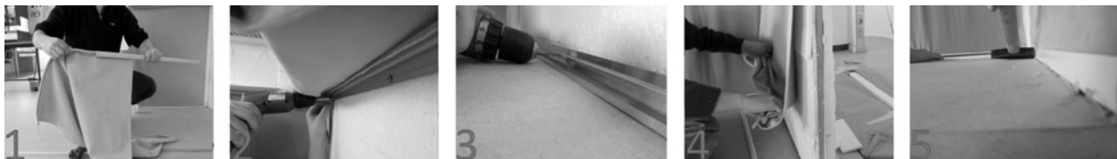
Fig. 1. Sequence of assembly, solution no. 1: 1 - inserting fabric with Keder bar in the upper profile; 2 - fixing the upper profile; 3 - fixing the lower profile; 4 - fabric tensioning; 5 - fabric fixing at the bottom edge.
