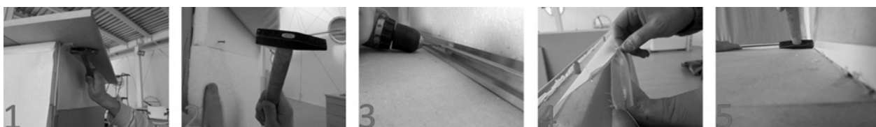
Fig. 2. Sequence of assembly, solution no. 2: 1 - fixing the PVC strip to the wall; 2 - installing the insulation layer in front of the PVC strip; 3 - fixing the lower profile; 4 - connecting the finishing fabric to the PVC strip with a plastic cursor; 5 - fabric fixing at the bottom edge.
